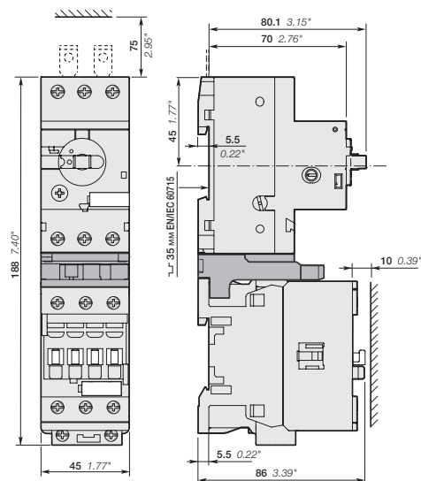
MS116-0.16-MS116-16 + BEA26-4 + AF26, AF30, AF38
