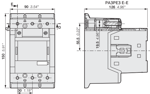
AF116, AF140, AF146-30-00
