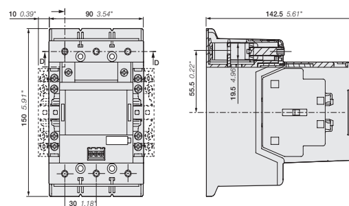
AF116, AF140, AF146-30-22
