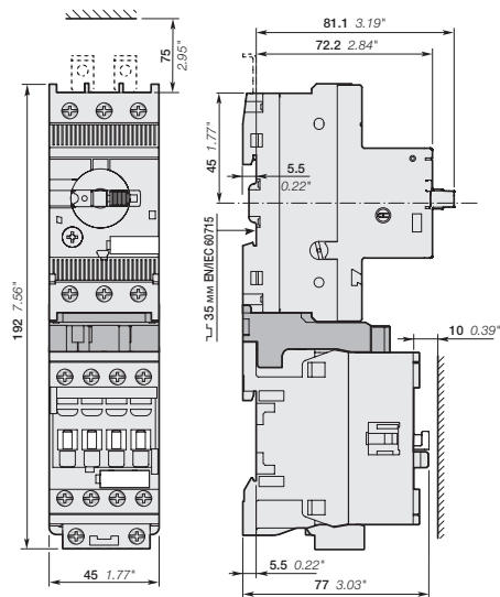
MS132-12-MS132-25 + BEA16-4 + AF09, AF12, AF16
